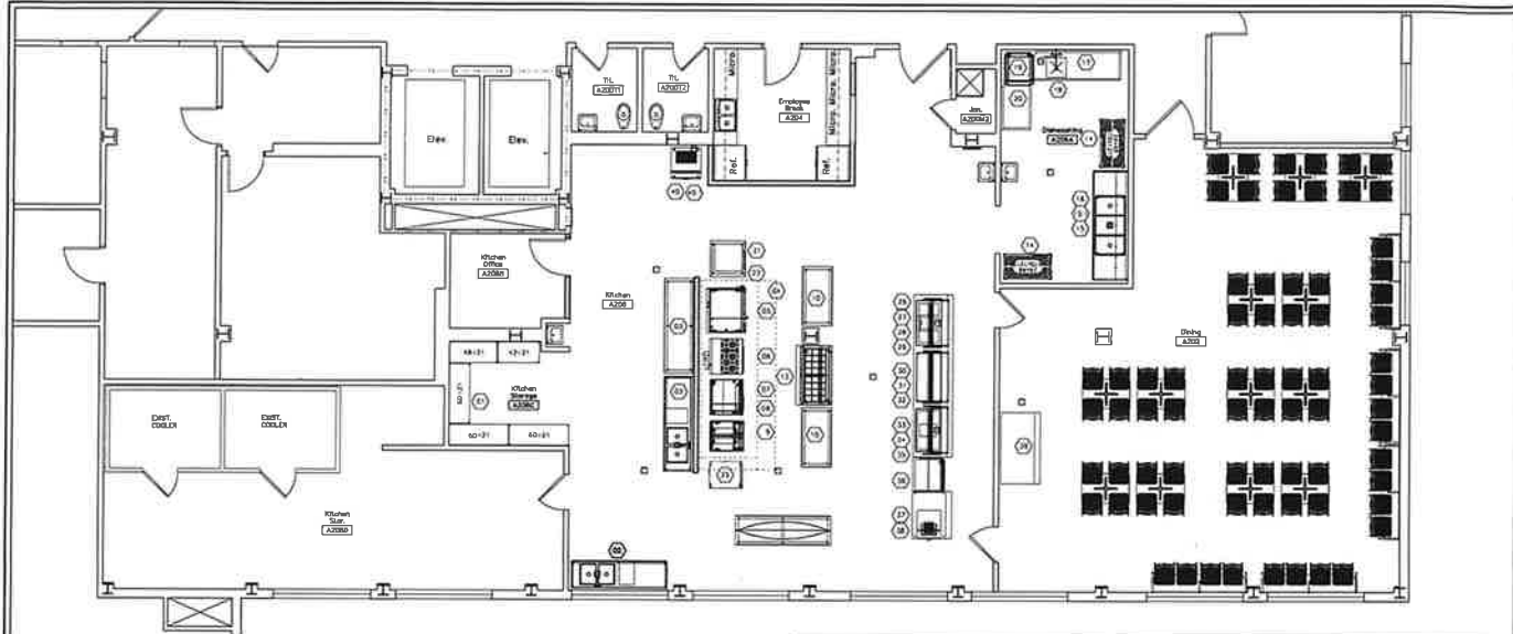
Kitchen Layout Second Floor Scale: 1/4" = 1'-0"
